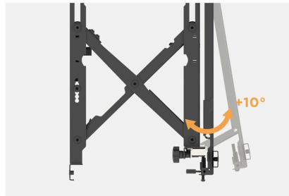
Kick-Stands provides 10° tilt for maintenance
