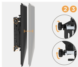
Depth Adjustment: +13.5mm rotating two knobs in the same direction
